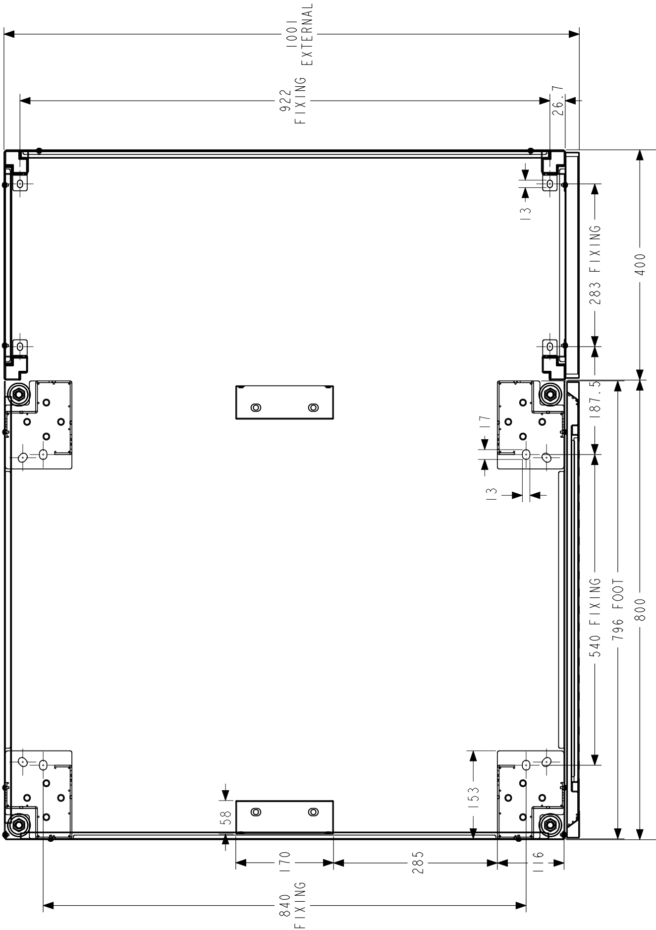
13.5. Drawing 5: DELPHYS XM 300 to 600 kVA bottom connection floor-mounted
